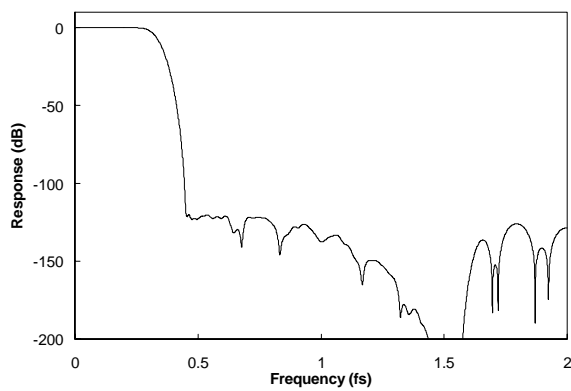
Figure 44 Medium Rate PCM Filter 4 Frequency Response
