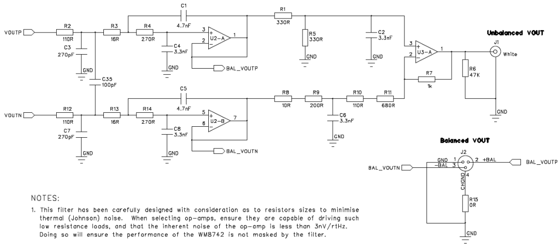
Figure 82 External Components
