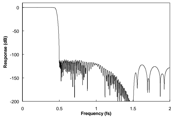
Figure 42 Medium Rate PCM Filter 3 Frequency Response
